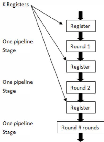
Fig. 3. Pipeline method [8].
