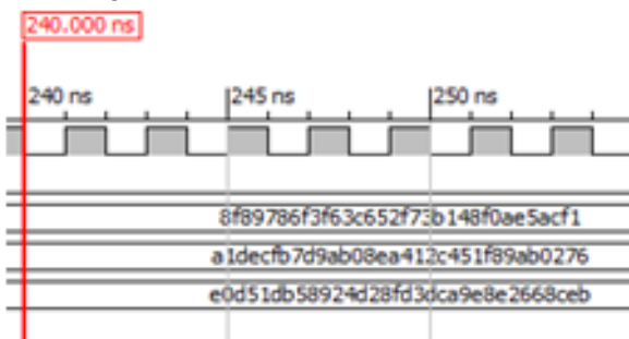
Fig. 4. Simulation result.
