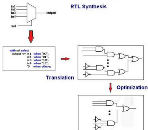
Fig. 1. Software optimization.
