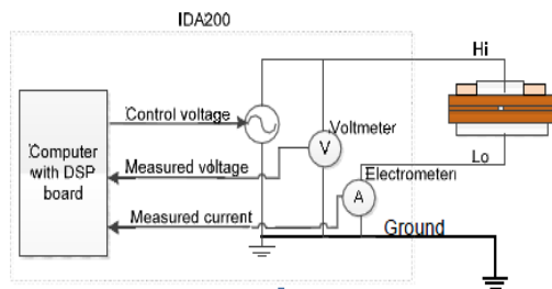
Fig3. Schematic diagram of spectrometric measuring system.
