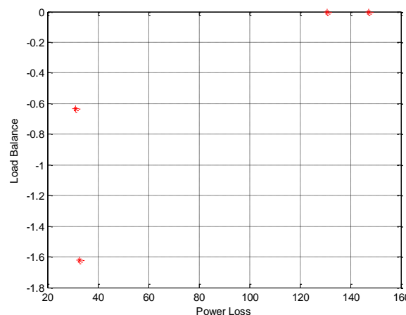
Figure 10: Pareto's response to simultaneous reconfiguration in the presence of DG
