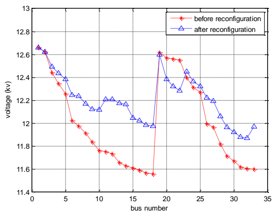
Figure 3. Comparison of the voltage profile curve before and after the reconfiguration with the aim of reducing losses without DG
