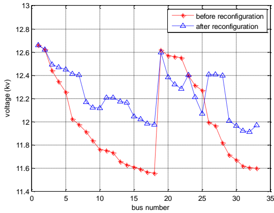
Figure 7: curve of Voltage profile before and after simultaneous rearrangement without DG
