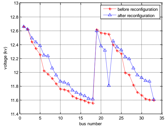
Figure 6. Comparison of the voltage profile curve before and after the reconfiguration with the load balancing target in DG presence
