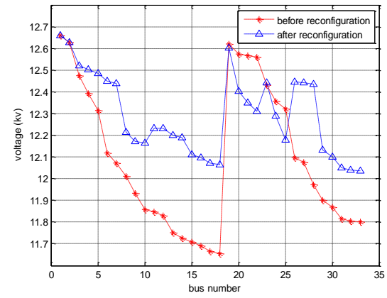
Figure 8: Voltage profile curve before and after simultaneous reconfiguration in DG presence
