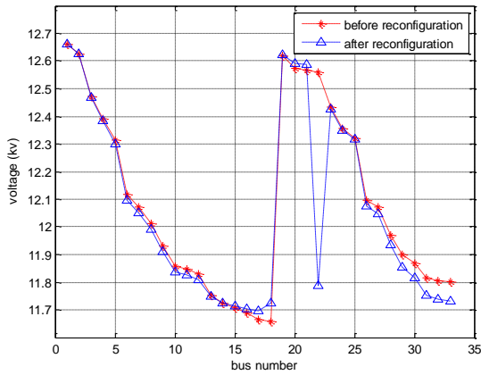
Figure 5. Comparison of the voltage profile curve before and after the reconfiguration with the aim of load balancing without DG
