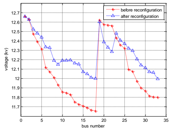
Figure 4. Comparison of the voltage profile curve before and after the reconfiguration with the aim of reducing the losses in the presence of DG
